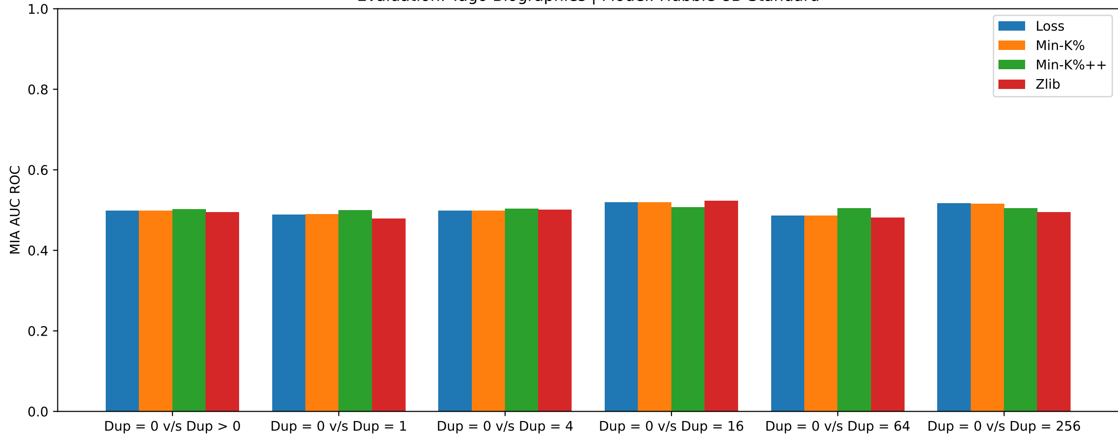
Evaluation: Yago Biographies | Model: Hubble-8B-Standard
